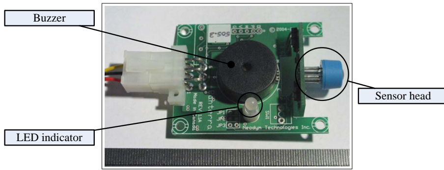
Figure 3: Panterra-CAT, uses the catalytic bead sensing principle.
