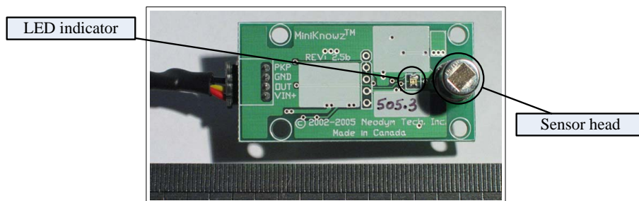
Figure 2: MiniKnowz, uses the metal-oxide semiconductor sensing principle.
